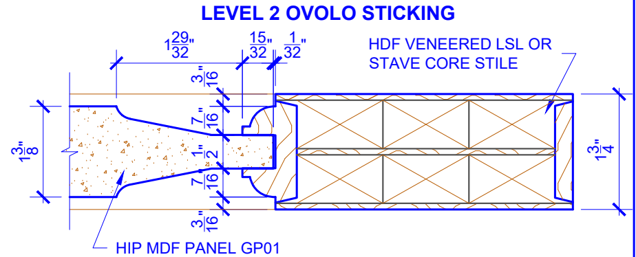
DETAIL 1
