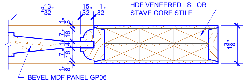
DETAIL 2
