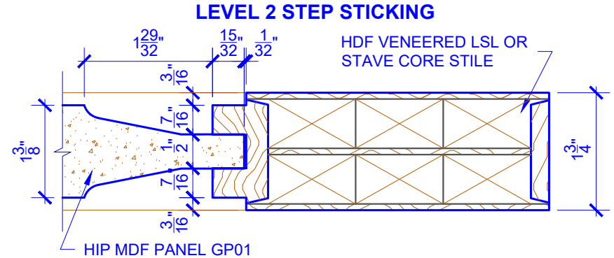
DETAIL 1
