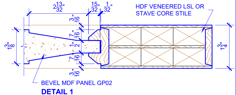
DETAIL 1
