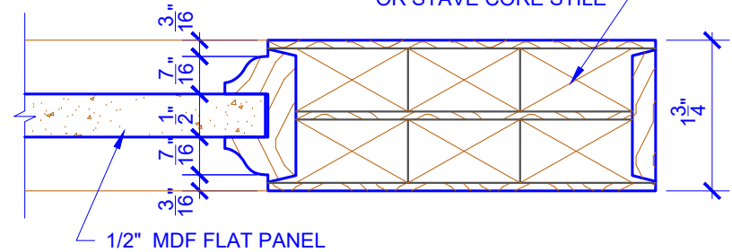
DETAIL 1
