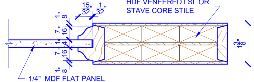
DETAIL 2
