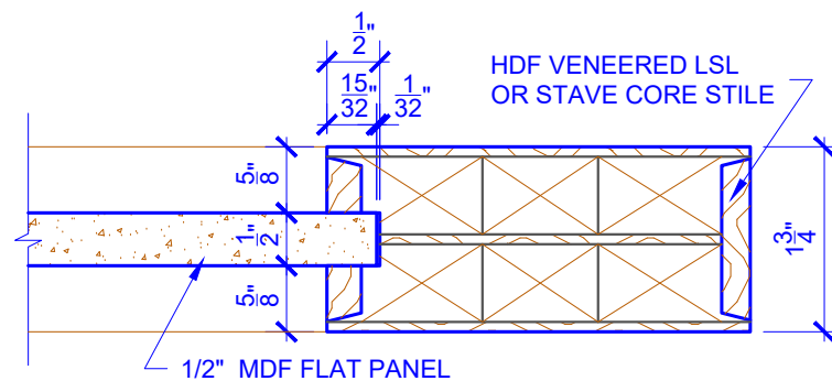
DETAIL 1
